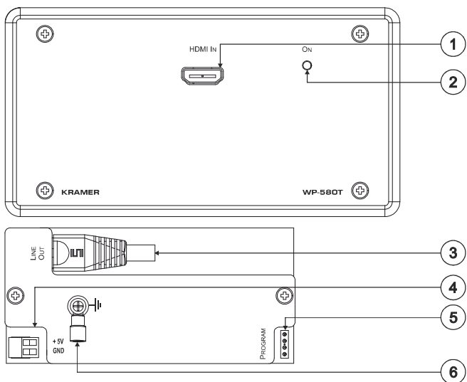
Figure 2: WP-580T HDMI Line Transmitter for Europe (80mm/86mm)
