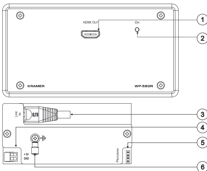
Figure 4: WP-580R HDMI Line Receiver for Europe (80mm/86mm)
