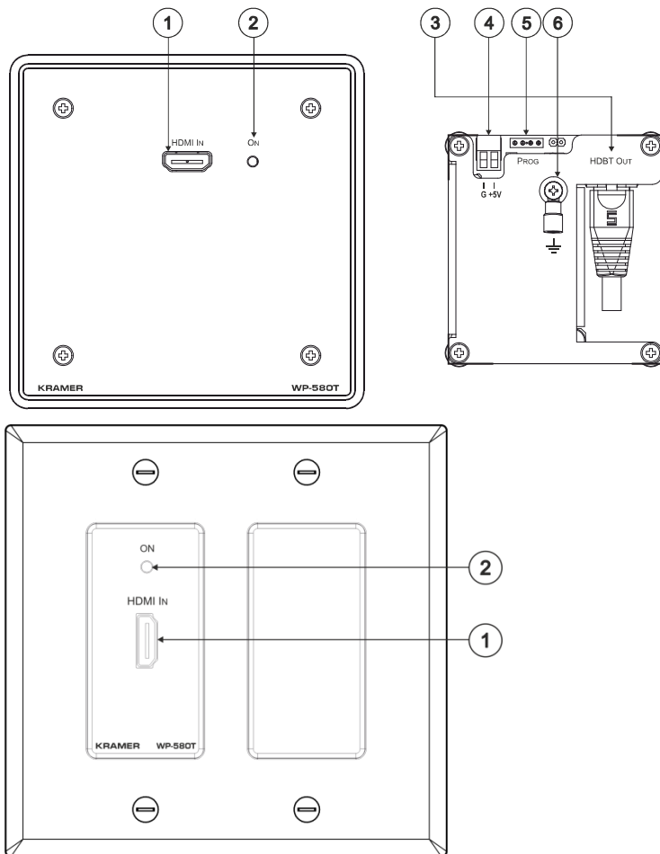
Figure 1: WP-580T HDMI Line Transmitter for the US and Decora®
