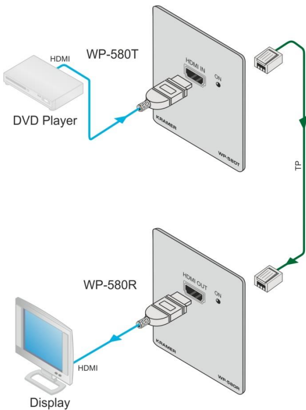
Figure 5: Connecting the WP-580T/WP-580R Transmitter/Receiver
