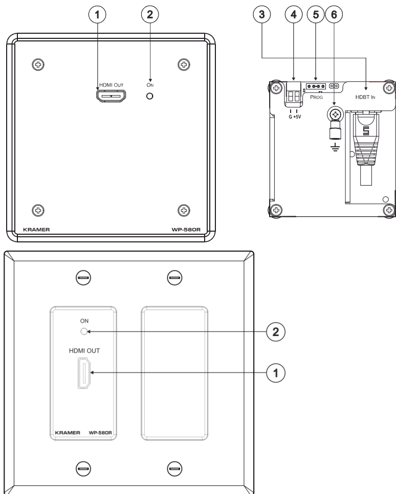
Figure 3: WP-580R HDMI Line Receiver for the US and Decora®
