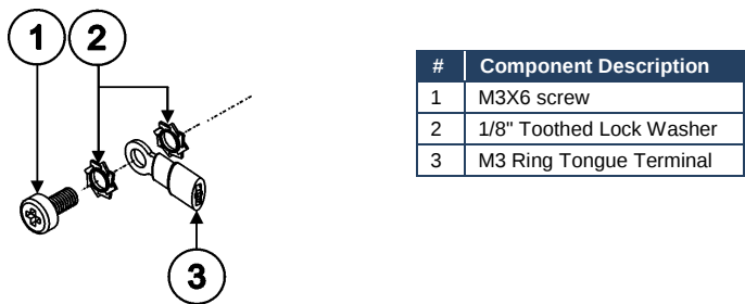
Figure 7: Grounding Connection Components
