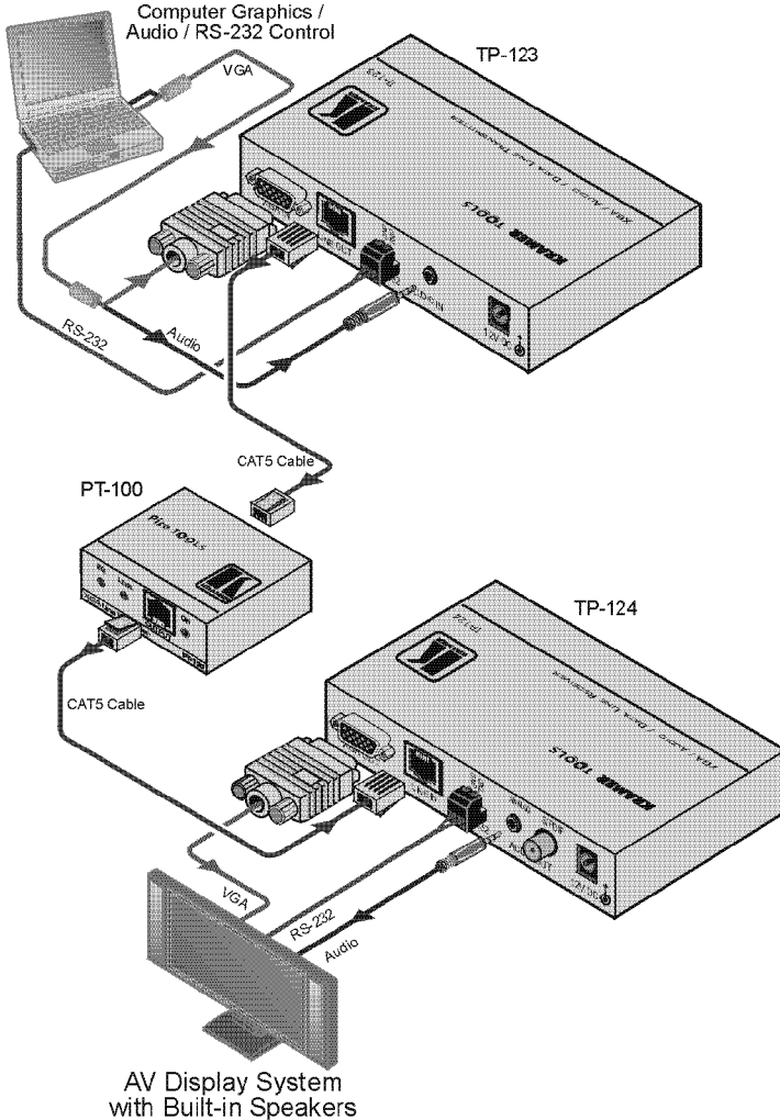
Figure 3: Connecting the PT-100 as a Simple TP Line Extender
