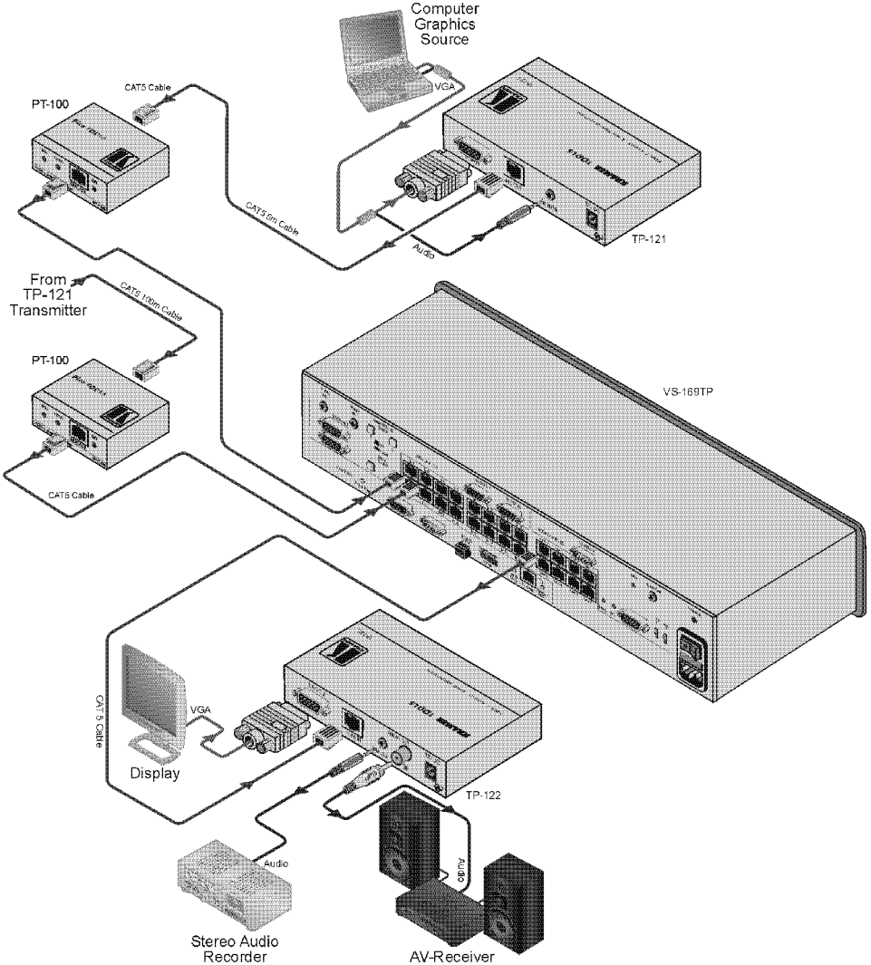
Figure 2: Connecting the PT-100 XGA Line Extender
