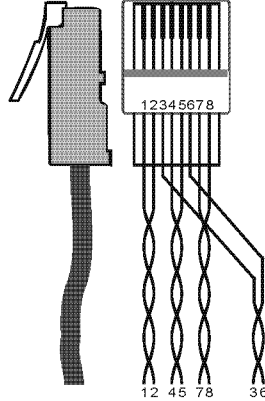
Figure 4: TP Connector
