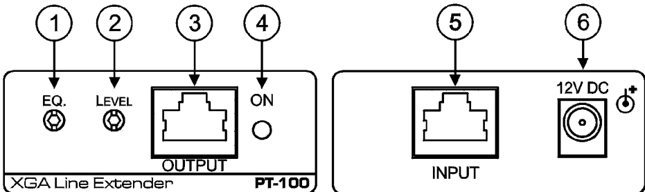
Figure 1: PT-100, XGA Line Extender Front and Rear Panels
