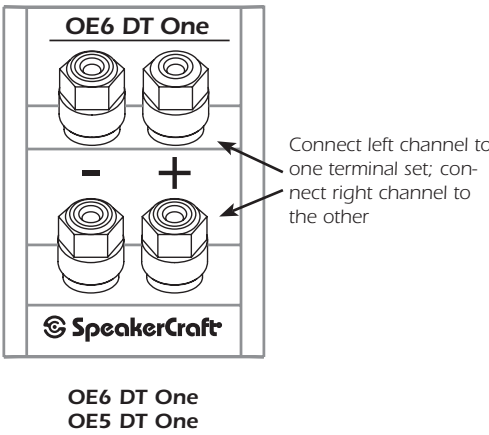
Diagram 2: DT Speaker Cable Terminals
