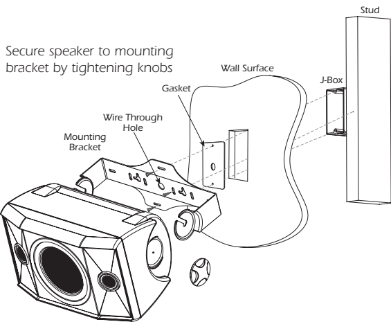
Diagram 4: Pre-Construction Installation
