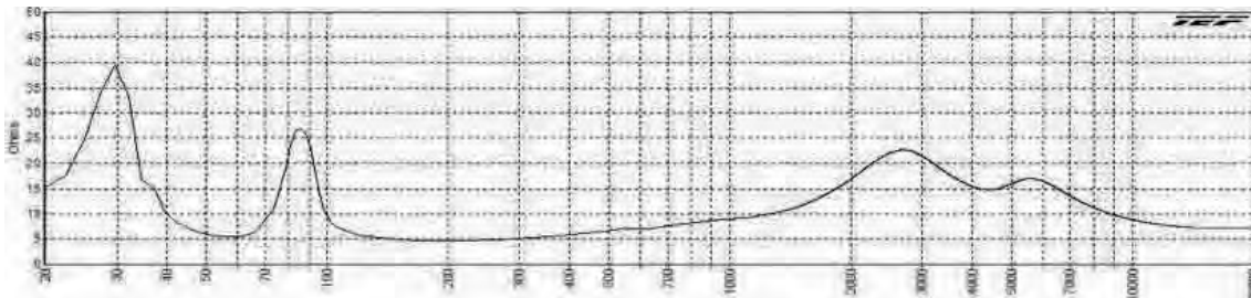
PM8CX Impedance
