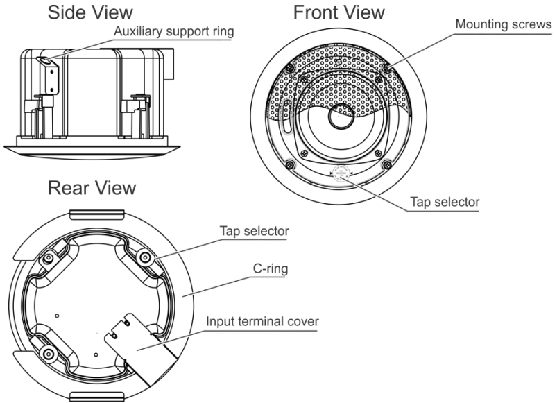
Figure 2: Galil 4-C Closed-back Ceiling Speaker
