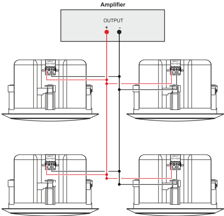
Figure 10: Square Layout Parallel Wiring
