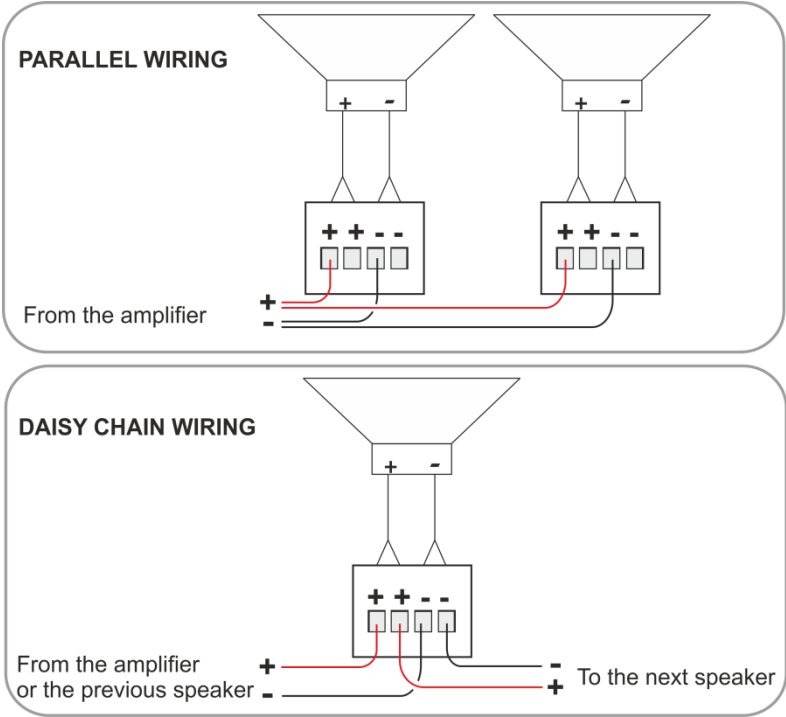
Figure 3: Closed-back Ceiling Speaker Schematic Diagram
