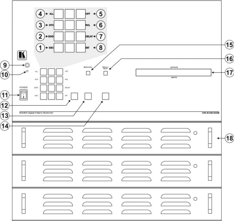
Figure 1: VS-6464DN 64x64 Digital Matrix Switcher
