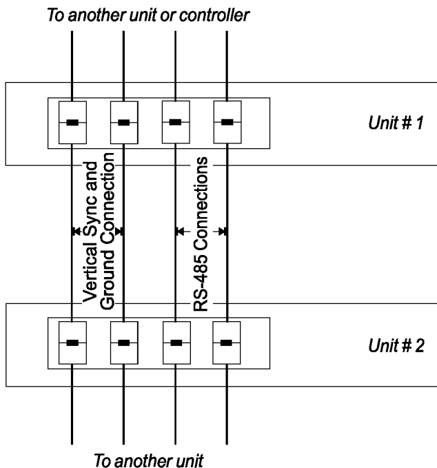
Figure 16: Connecting the RS 485 Connectors between 2 VS 162V Units
