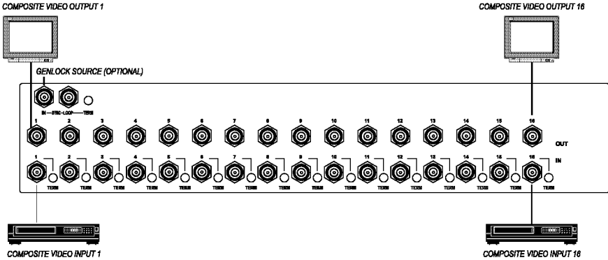
Figure 3: Configuring the VS 162V for Composite Video (CV)
