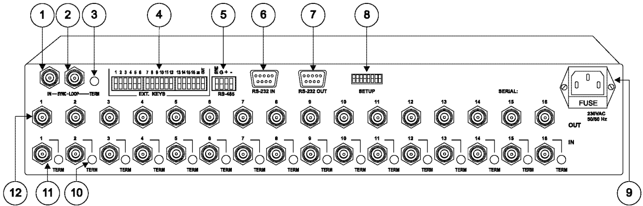
Figure 2: VS-162V 16x16 Video Matrix Switcher
