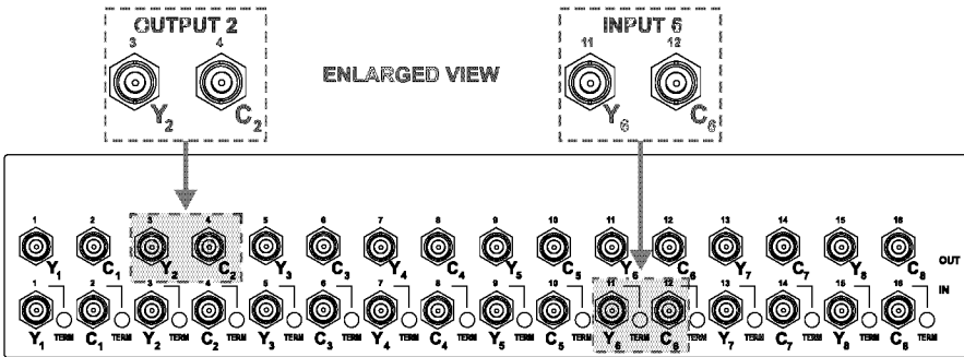
Figure 4: Configuring the VS 162V for s Video (Y/C)
