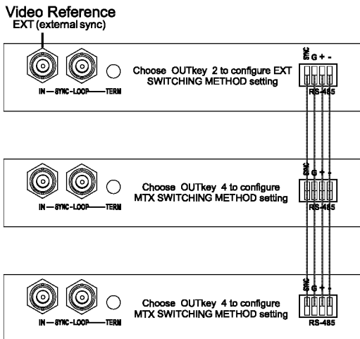
Figure 21: Choosing the MTX (SYNC from Matrix) Setting
