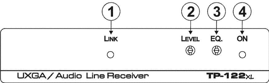
Figure 3: TP-122xl UXGA/Audio Line Receiver Front Panel
