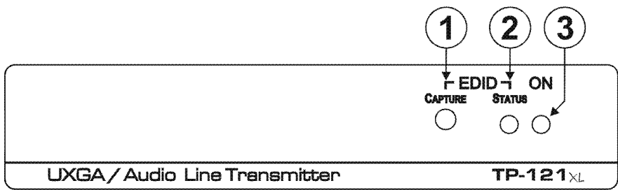
Figure 1: TP-121xl UXGA/Audio Line Transmitter Front Panel
