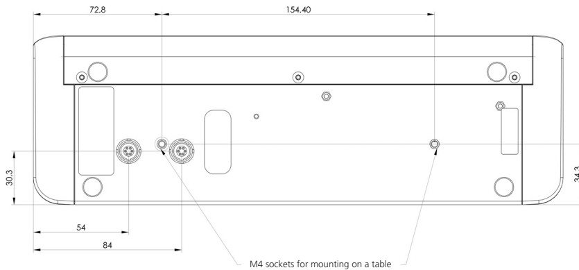
Bottom view H-version
