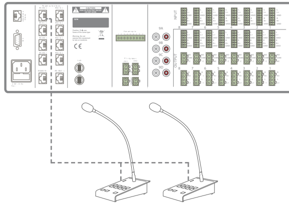
Multiple paging consoles connected on one PI port (Bus structure)
