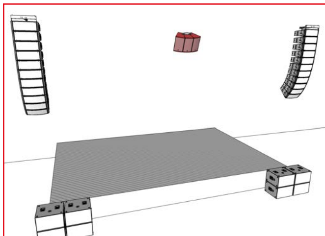
Complement to large PA Systems - Flown Center-fill
