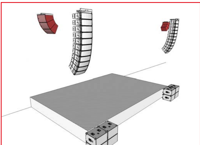
Complement to large PA Systems - Flown Out-fill
