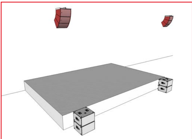
Main PA System - Flown Vertical Array
