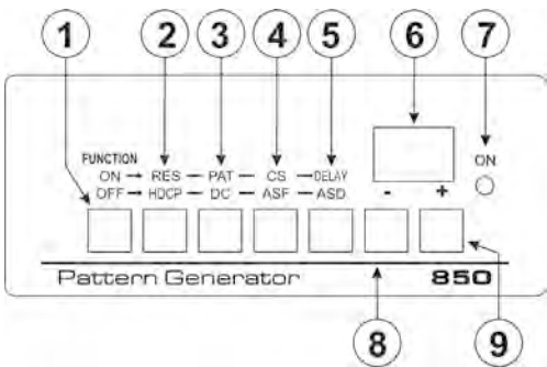
Figure 1: 850 Pattern Generator Front Panel
