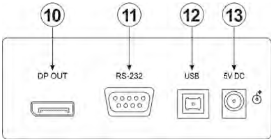
Figure 2: 850 Pattern Generator Rear Panel
