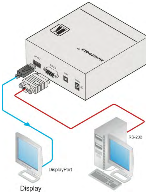
Figure 3: Connecting the 850 Pattern Generator
