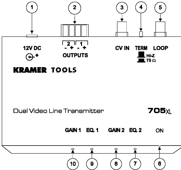
Figure 2: 705xl Dual Video Line Transmitter
