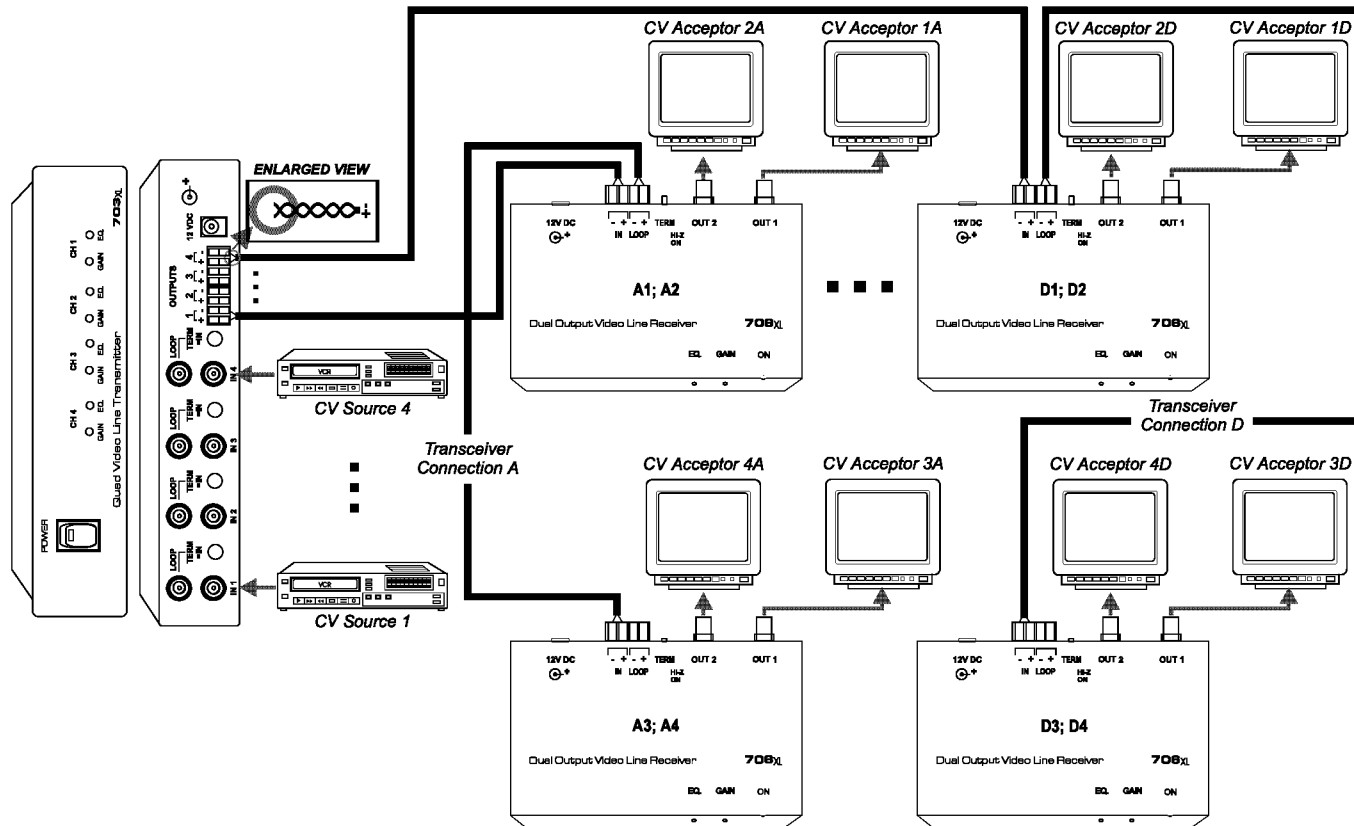
Figure 5: 703xl Quad Video Line Transmitter / Receiver System
