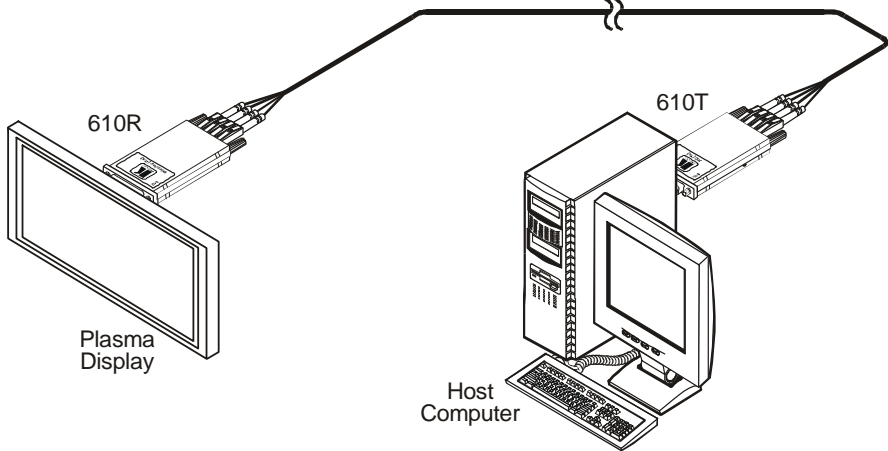
Figure 3: Connecting the 610T/610R Detachable Optical DVI Transmitter/Receiver
