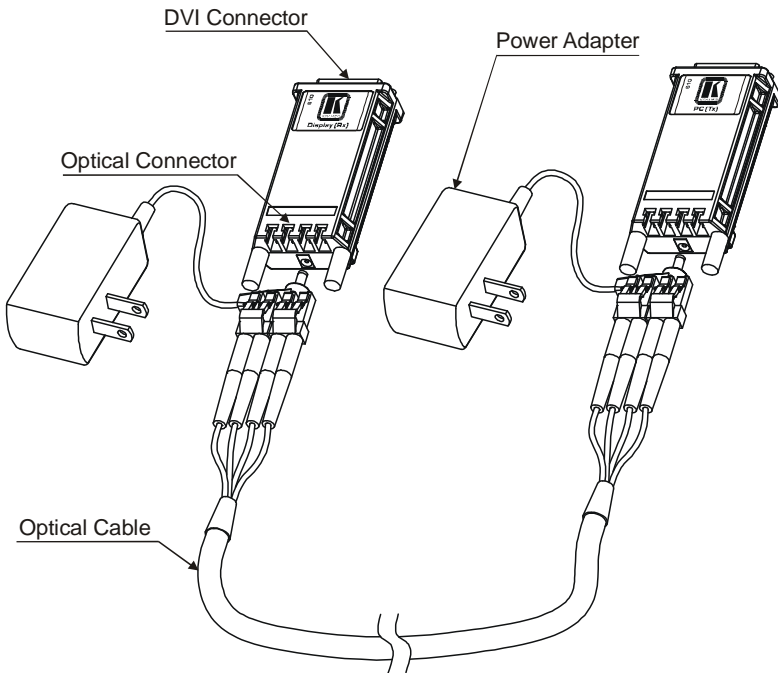
Figure 1: 610 Detachable Optical DVI Transmitter and Receiver
