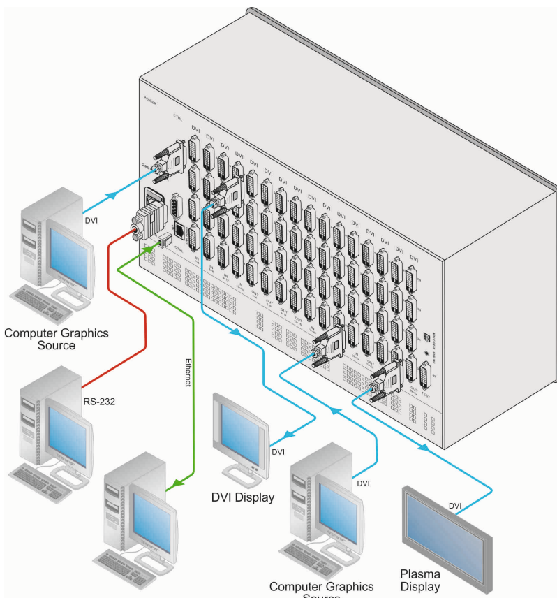
Figure 4: Connecting the VS-3232DN
