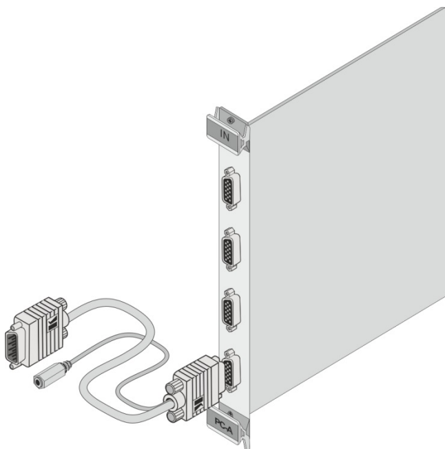
Figure 16: Accessing Audio over VGA
