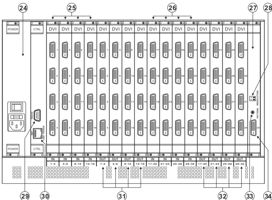
Figure 3: VS-3232DN Rear Panel Showing DVI cards
