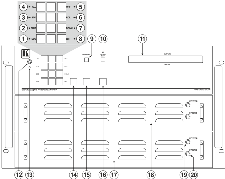
Figure 1: VS-3232DN Front Panel
