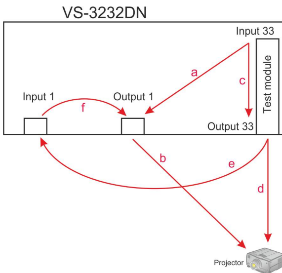
Figure 17: Signal Paths for Isolating Video Problems
