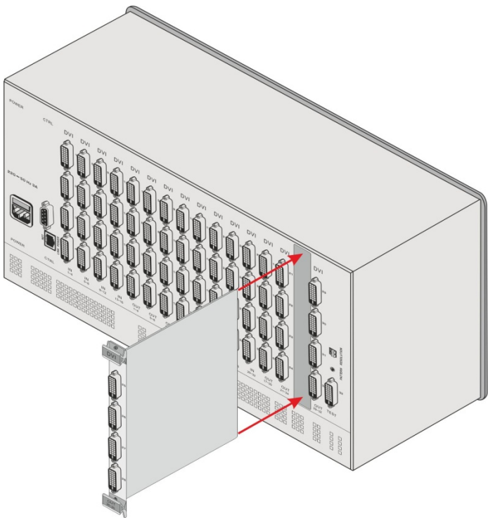
Figure 18: Inserting the Card into a Slot
